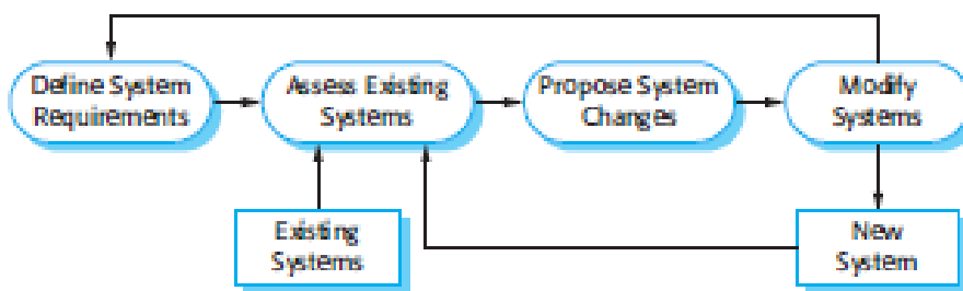
Fig 1.15: System Evolution
