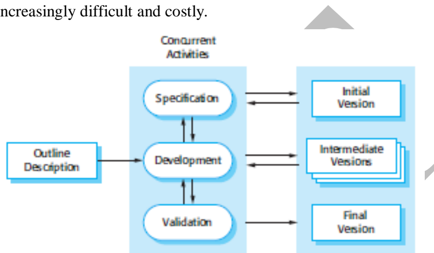
Fig 1.9: Incremental Development
