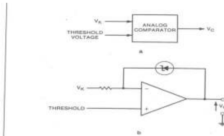
Knock Level Detector Circuit
