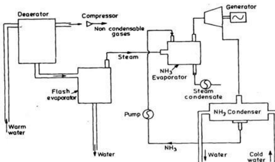
Fig. Hybrid Cycle
