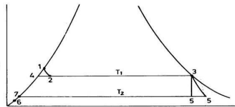
OPEN CYCLE OTEC SYSTEM (CLAUDE CYCLE)
