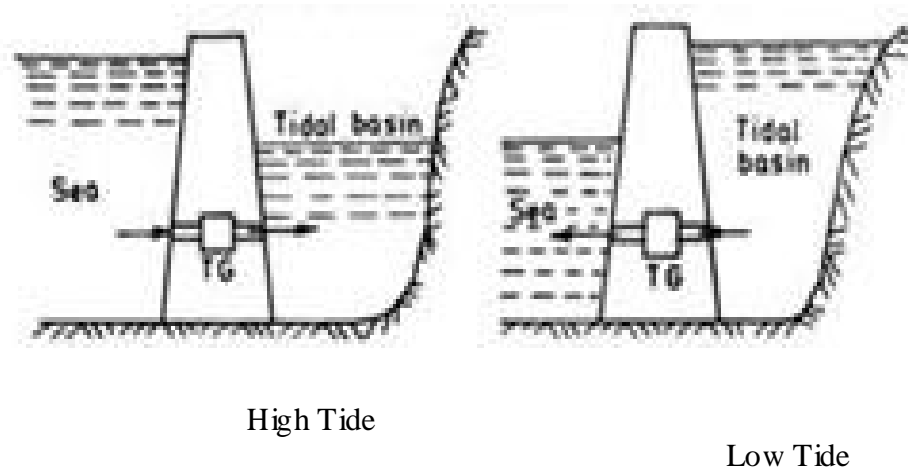
Fig. Double Cycle System
