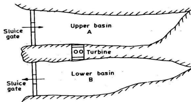
Fig. Tidal power plant Double Basin Operation.
