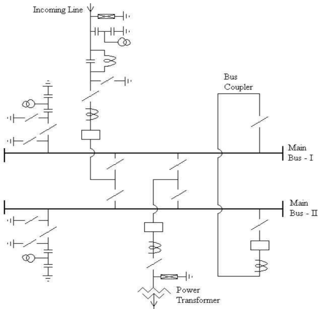
TYPICAL DOUBLE BUS BAR ARRANGEMENT
