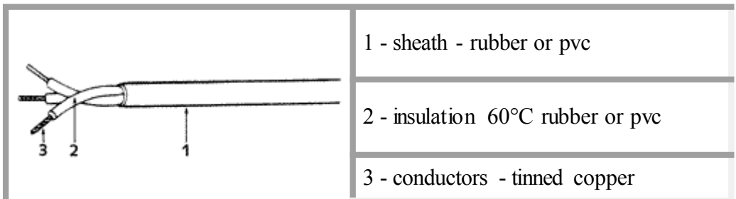
c) Circular sheathed - Fig 4.2c
