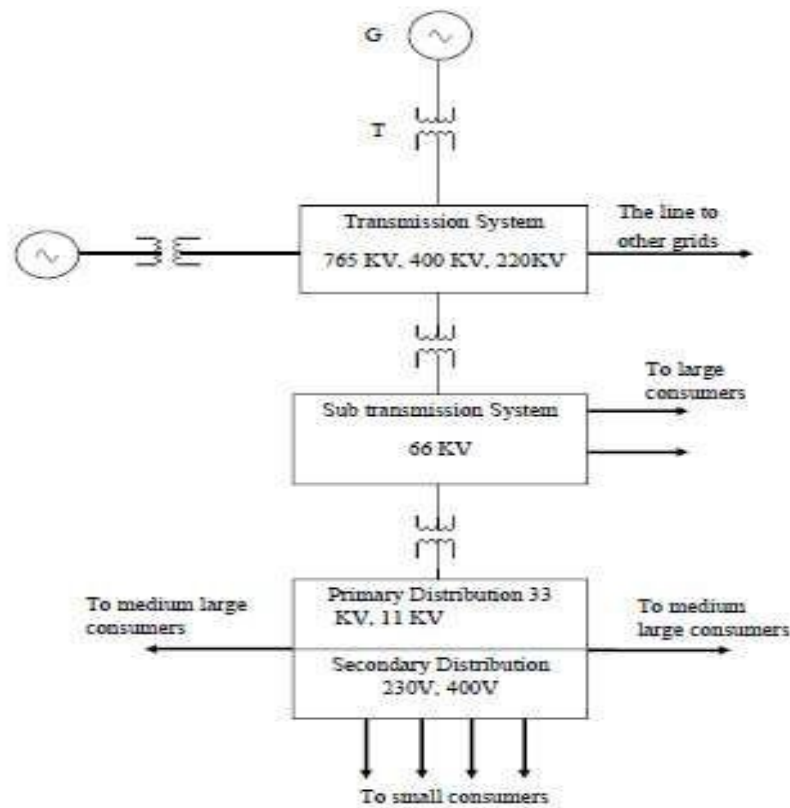
Figure 1.1 Single line Power System Network
