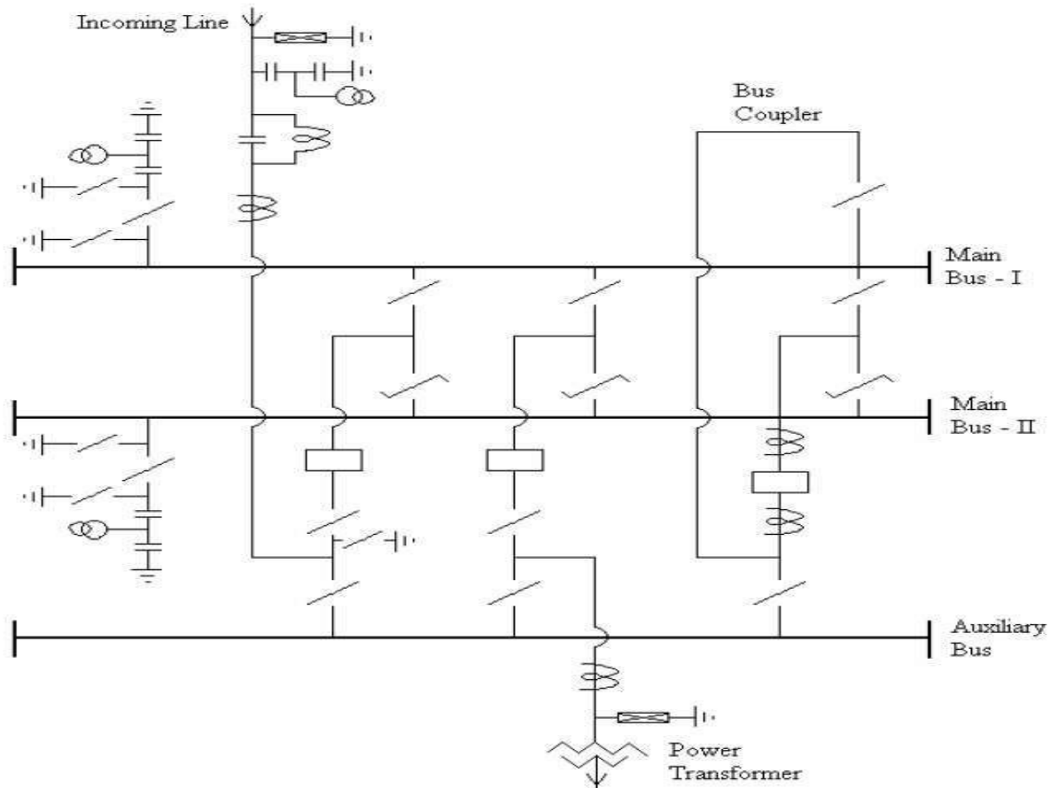
TYPICAL DOUBLE MAIN AND AUXILIARY BUS BAR ARRANGEMENT
